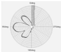
G-8 5.8 GHz antenna vertical plane pattern
