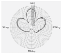
G-8 5.8 GHz antenna azimuth plane pattern
